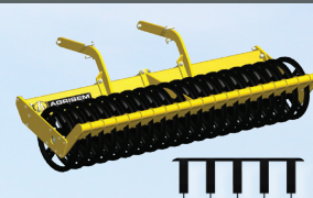
Steel-Pack Ø700
